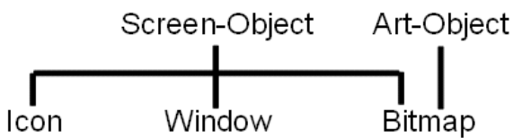
Figure 1.10. Multiple Inheritance
