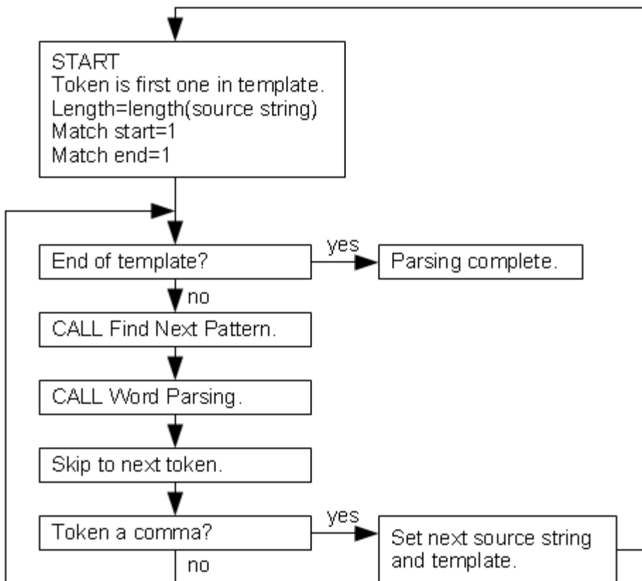
Figure 9.1. Conceptual Overview of Parsing
